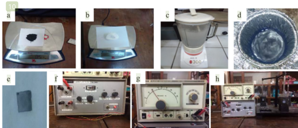
Figure 4: Illustrations of (a) weighing graphite powder; (b) weighing detergent powder; (c) blender for mixing the materials; (d) shallow dish for samples of the solutions after sonication treatment; (e) sample on the glass slide after annealing; (f) Uchida TA-2MS amplifier; (g) CSi/SPECO SS-1 audio generator; and (h) assembly of the self-custom-made ultrasound generator and submerging the probes into the solution.
