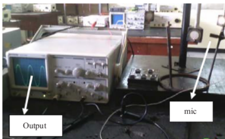
Figure 3: A validation activity of the signal output produced by the piezoelectric compared to the given frequency of the audio generator. The mic condenser (on the right) is placed in front of the piezoelectric. The output signal may be observed by an oscilloscope.
